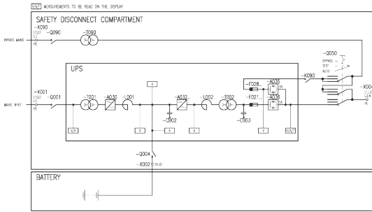
Single phase drawing
